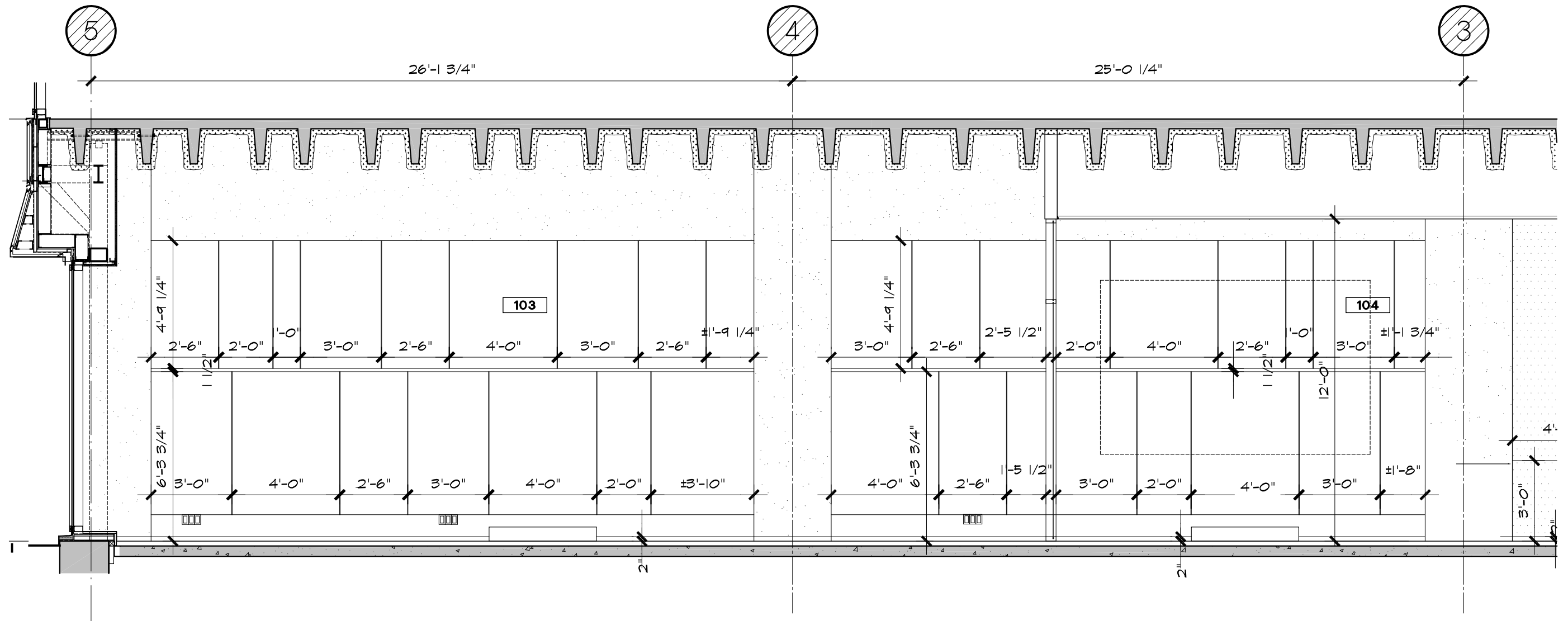
1 ELEVATION INTERIEURE A2.1 LOCAL 103 ECHELLE 1:50
